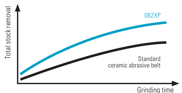
Dry grinding of wire to remove forge scale
